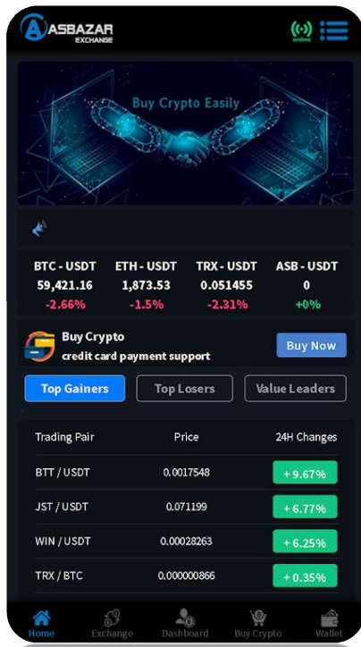
Application interface
